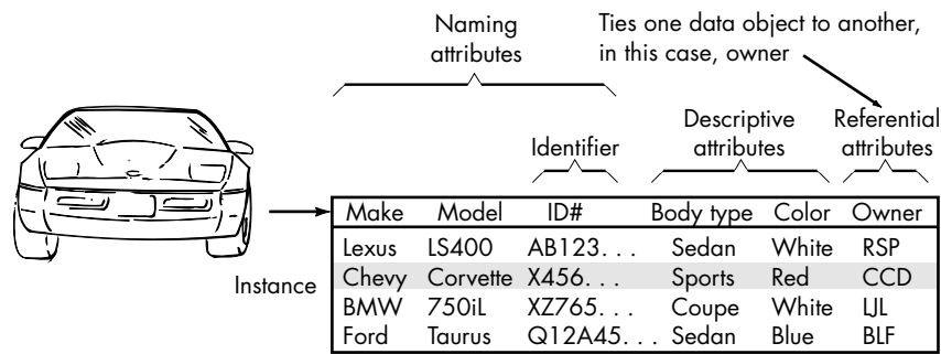
FIGURE 12.3 Tabular representation of data objects
