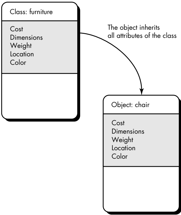
FIGURE 20.2 Inheritance from class to object
